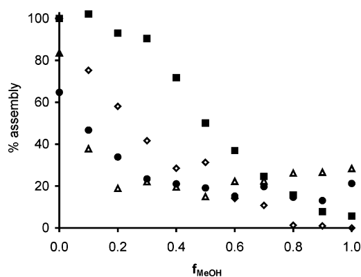
Fig. 8 CD titrations of assemblies 7a ,(( R )-PhEtCYA) 6 (■), 7b ,(BuCYA) 6 (◇), 7d ,(BuCYA) 6 (Δ) and 7e ,(BuCYA) 6 (●). Spectra were recorded in MeOH–CHCl 3 ( f_{\text{MeOH}} ) mixtures at 298 K where the maximum assembly concentration was kept constant (1.0 mM).
