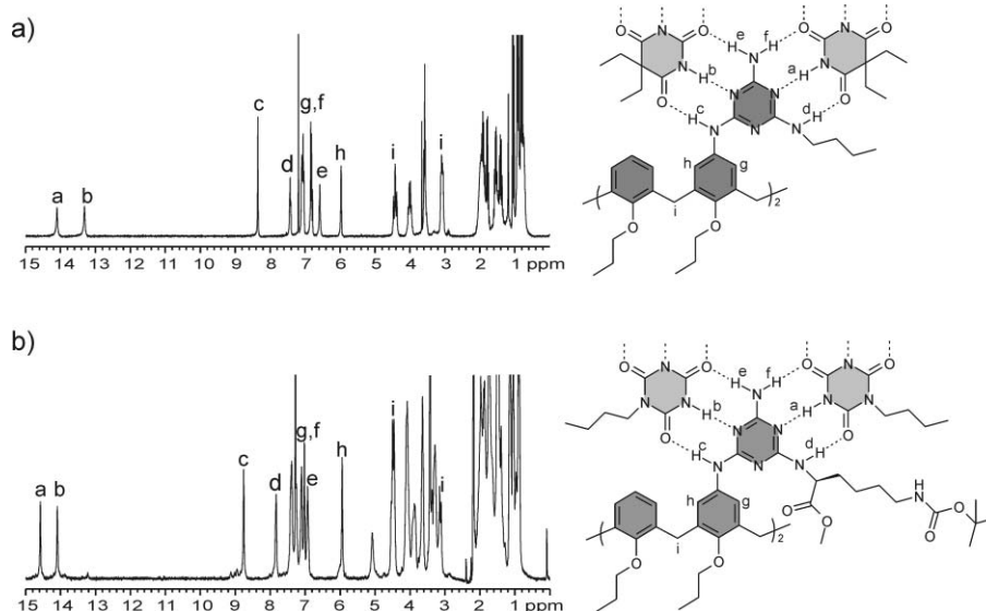
Fig. 3 1 H NMR spectra of assembly (a) 1a 3 ·(DEB) 6 and (b) 6d 3 ·(BuCYA) 6 . Spectra were recorded at 300 MHz in CDCl 3 at 298 K. (For clarity only the molecular structure of part of one rosette floor of the assemblies is shown).
