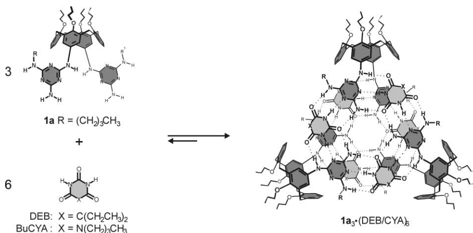
Fig. 2 Formation of the double rosette assemblies 1a_3 \cdot (DEB/BuCYA)_6 from three calix[4]arene dimelamines 1a and six 5,5-diethylbarbiturate (DEB) or n -butyl cyanurate (BuCYA) molecules.
